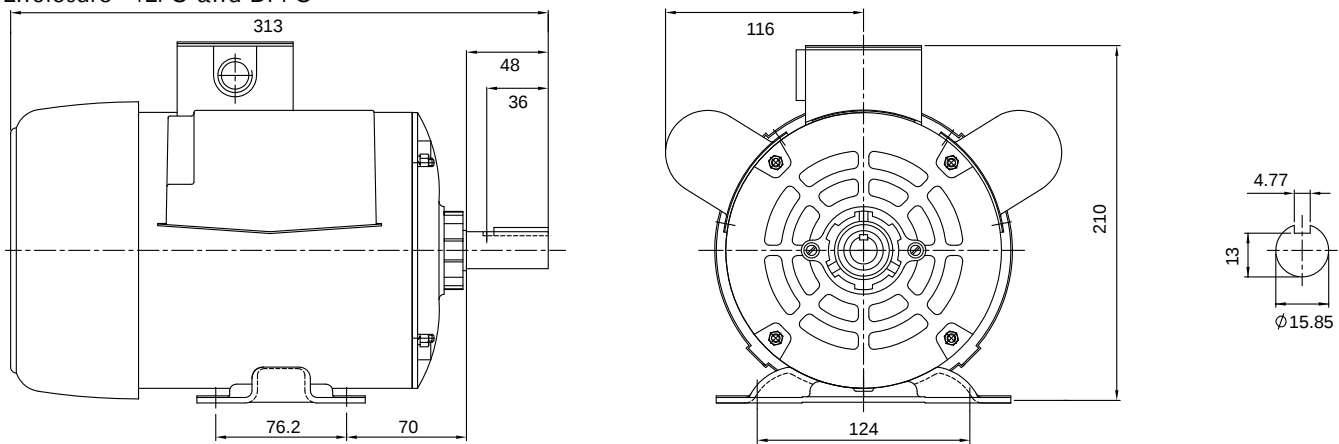
Enclosure - DP
